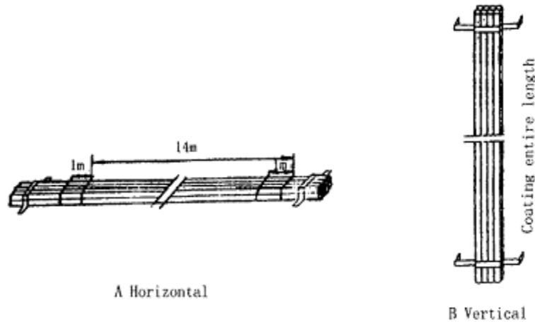
Fig 2.12.10.4 Location of flameproof coatings
